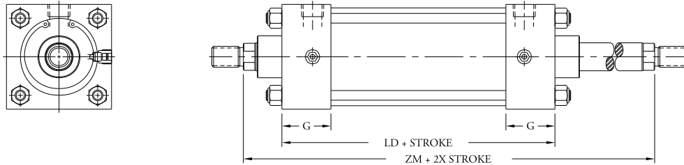
SERIES TDE/TMDE SERIES TSDE/TSMDE (oversized rod)
