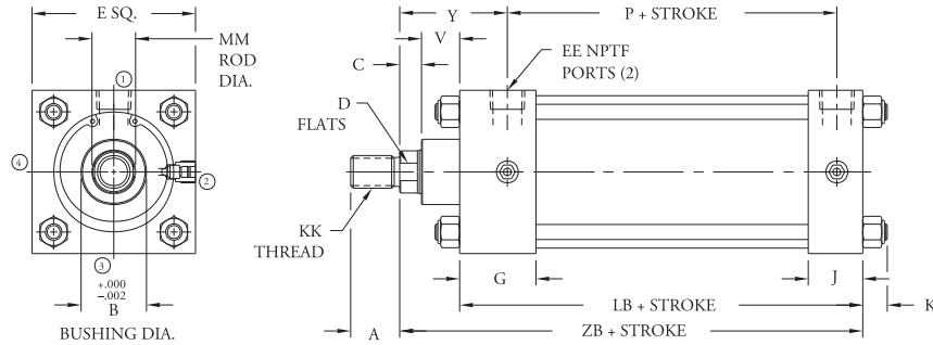
SERIES T/TM/TL SERIES TS/TSM/TLS (oversized rod)
