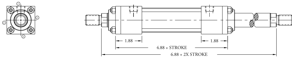
SERIES TSDE/TSMDE (1 1/2 BORE oversized rod)
