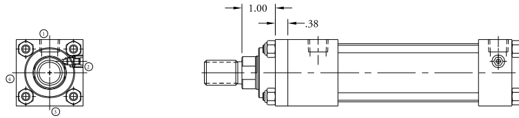
SERIES TS/TSM/TLS (1 1/2 BORE oversized rod)
