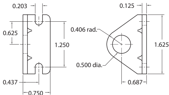
FB-1291 Foot Bracket Material: Steel, bright zinc plated
