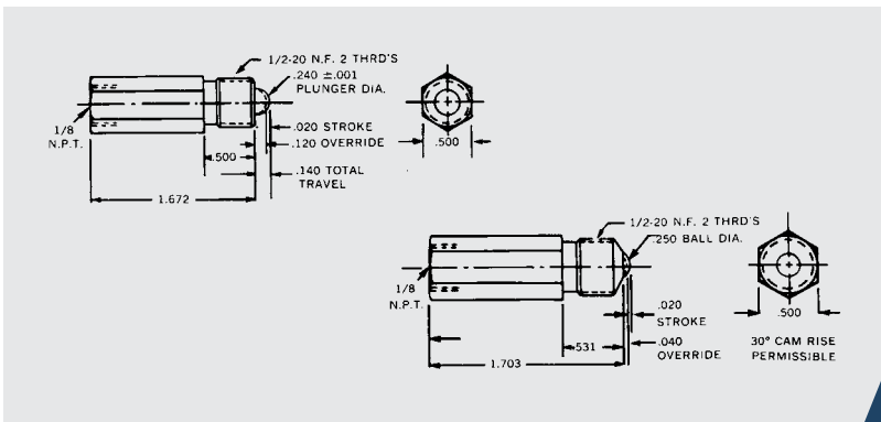
Model 7919 Air Bleeder Operated
