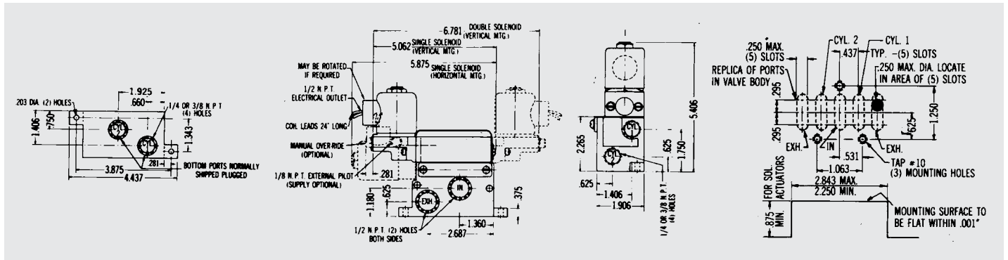
Multiple Station Manifolds
